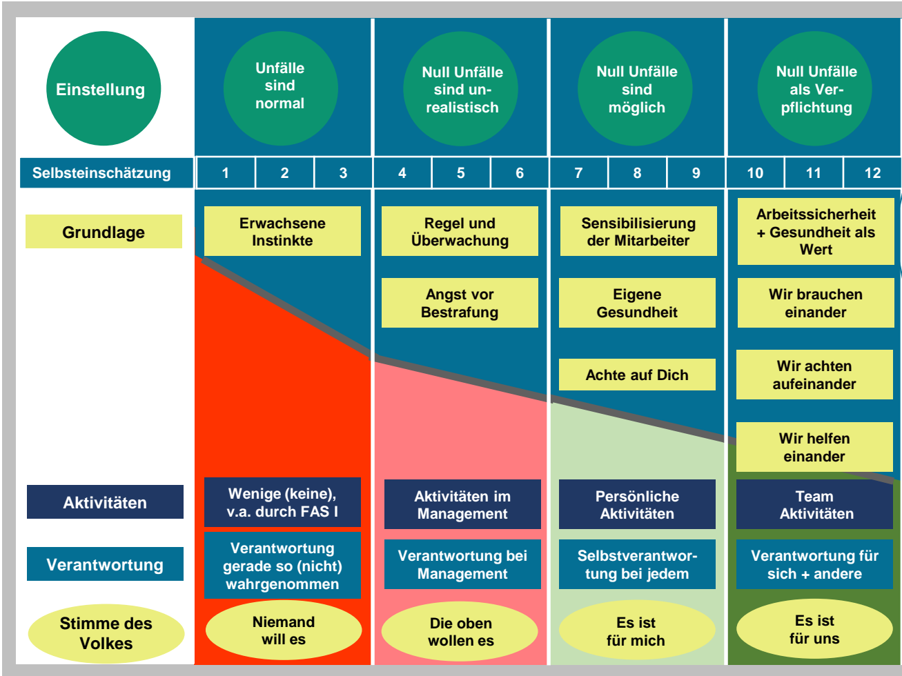
Bradley-Kurve
